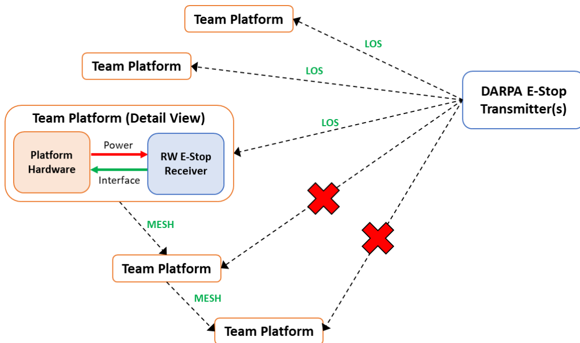
Figure 1: Concept of Operations for the Recovery Wireless E-Stop System
